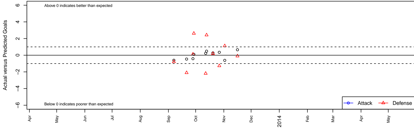
FC Golden State Gold B94 Dots are actual minus expected GF (blue circles) and GA (red triangles). Blue line is smoothed change in attack strength. Red is smoothed change in defense strength.
